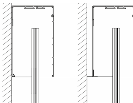
TYP C - Facade box. Dedicated F-FBR-010 guides.
